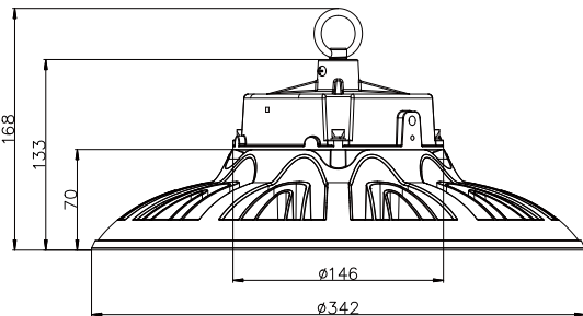
05 LGS-UFOB-300W
