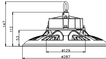
06 LGS-UFOB-400W/500W
