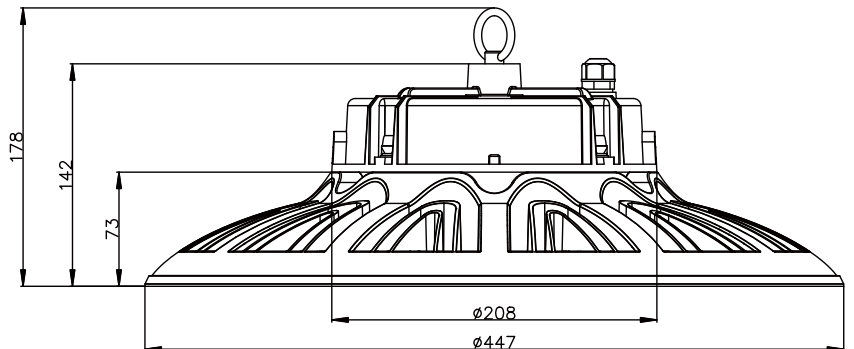
06 LGS-UFOB-400W/500W
