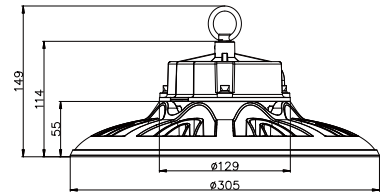
04 LGS-UFOB-200W/240W
